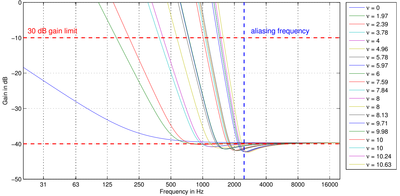
Figure 4: Radial filters for calculated orders \nu and radius a , gain limit, upper frequency limit for spatial aliasing
