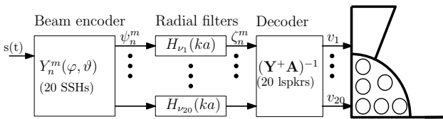
Figure 5: Block diagram of signal flow for modal beamforming
