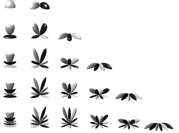
Figure 3: A set of 20 Spherical Sector Harmonics for values \mu_m and \nu_{nm} fulfilling the arrays geometrical boundary conditions
