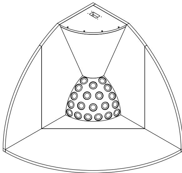
Figure 2: Design of the loudspeaker cabinet
